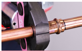
2. Complete the joint with the approved tool. Press once only
