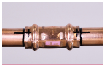
3. Mark the completed joint
