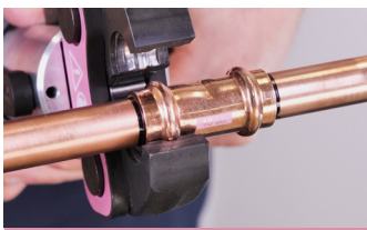
1. Align jaws squarely on the fitting
